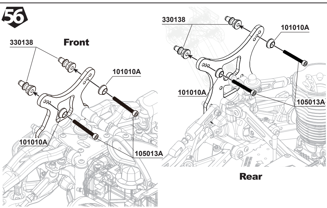
105013A M3x25mm Cap Screw x4
